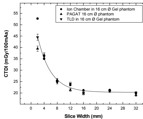
Figure 4. CTDI for various slice widths.
